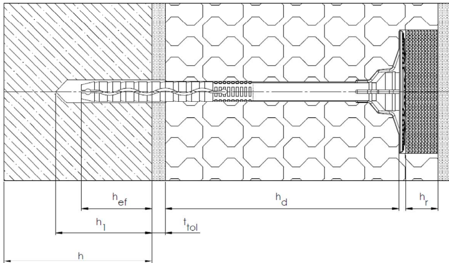
IMMERGED MOUNT
